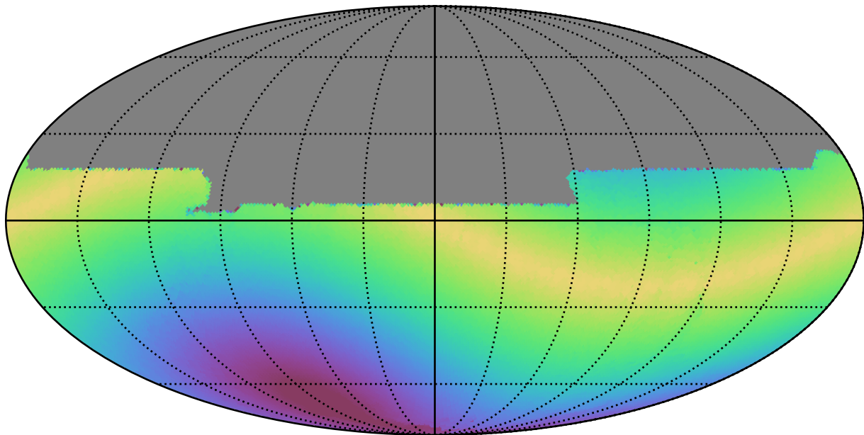
too_10_1v3.4_10yrs All sky y band: Max solarElong
