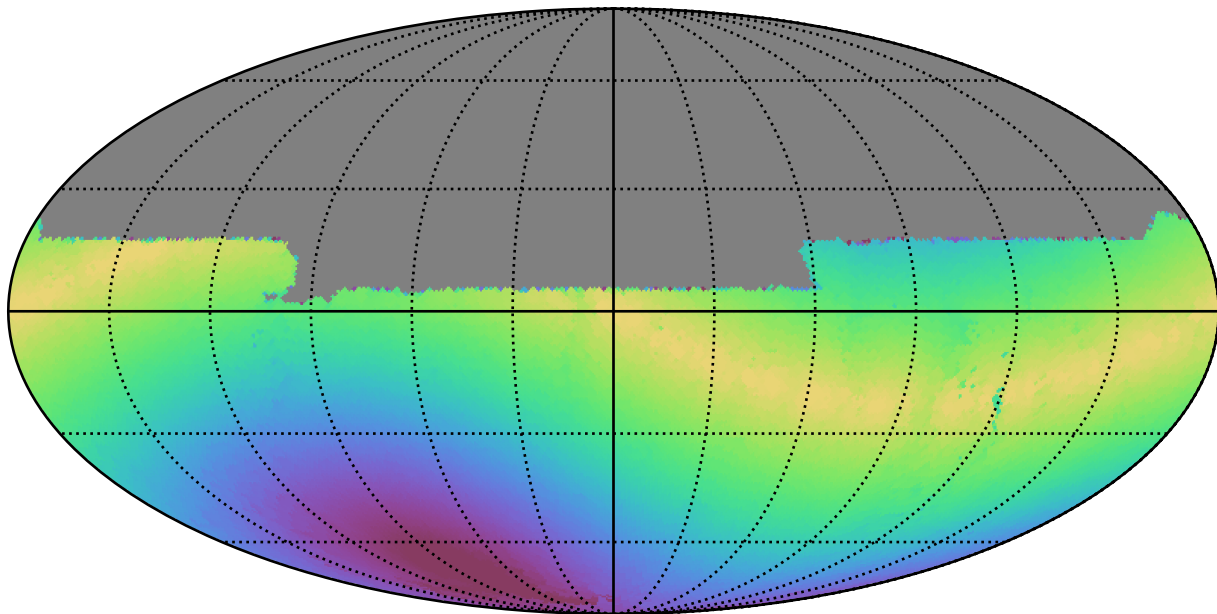
too_10_1v3.4_10yrs All sky u band: Max solarElong
