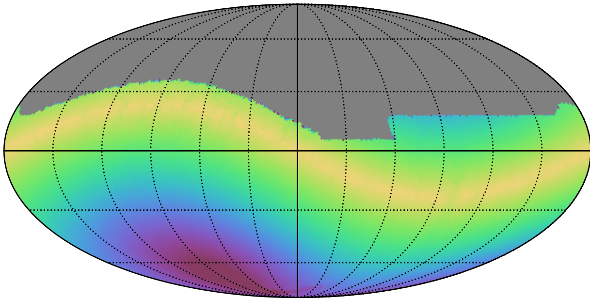
too_10_1v3.4_10yrs All sky r band: Max solarElong
