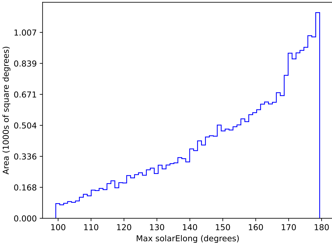
too_10_1v3.4_10yrs All sky r band: Max solarElong
