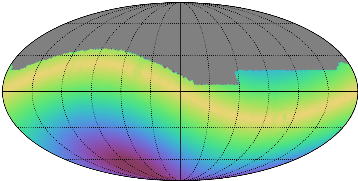
too_10_1v3.4_10yrs All sky i band: Max solarElong
