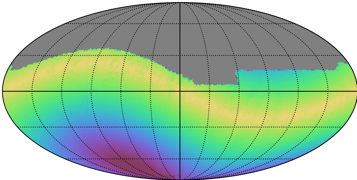
too_10_1v3.4_10yrs All sky g band: Max solarElong
