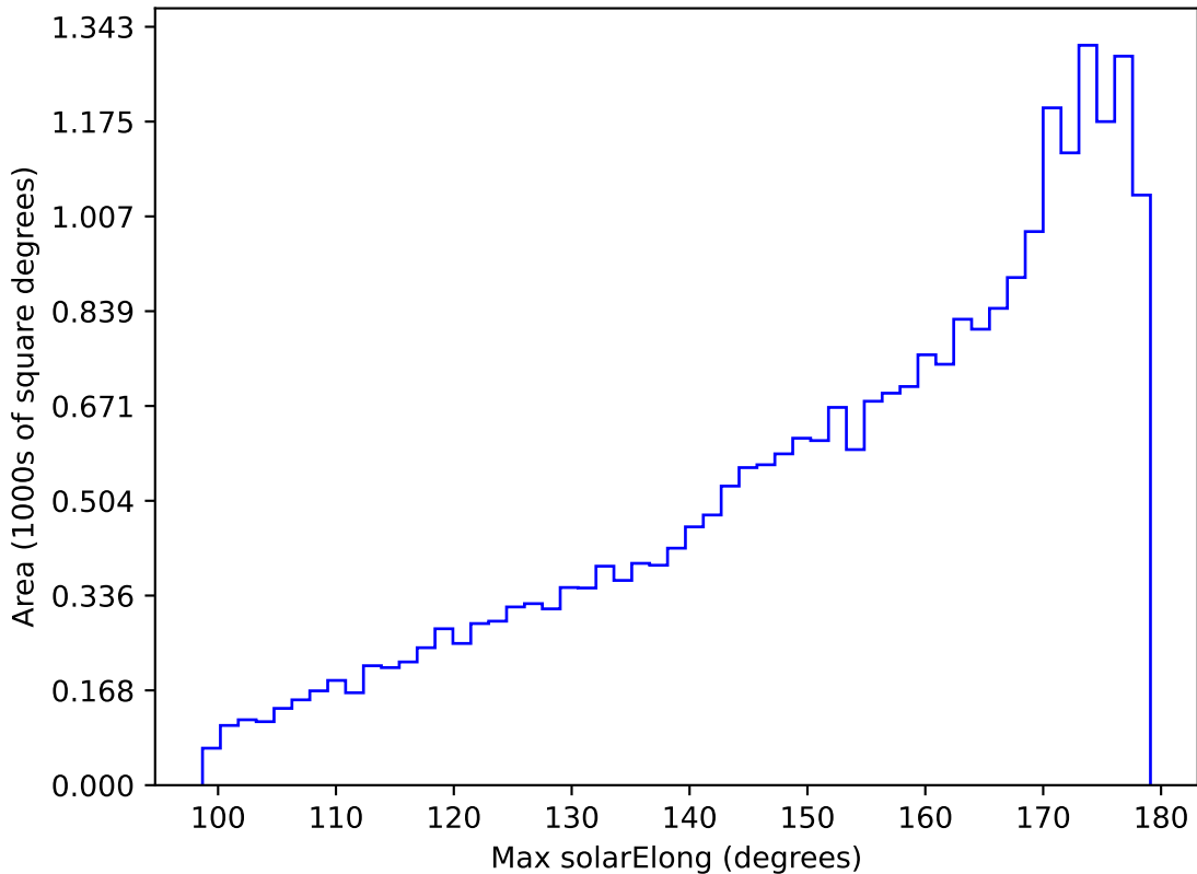
too_10_1v3.4_10yrs All sky g band: Max solarElong
