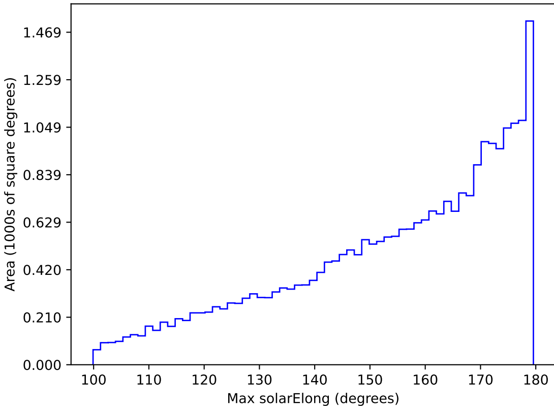
too_10_1v3.4_10yrs All sky all bands: Max solarElong
