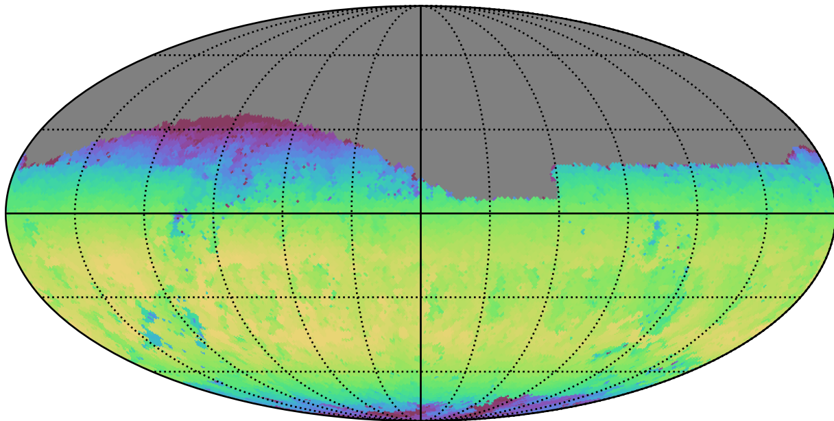
too_10_1v3.4_10yrs Yr 1 z band: Max skyBrightness
