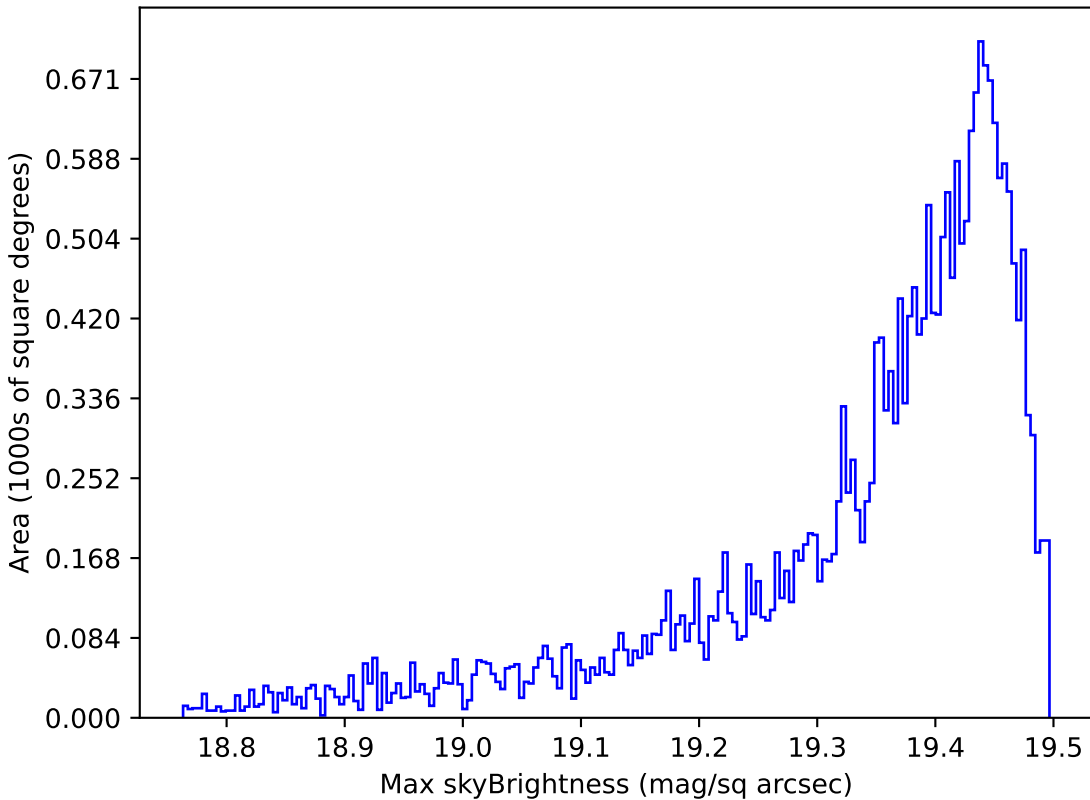
too_10_1v3.4_10yrs Yr 1 z band: Max skyBrightness
