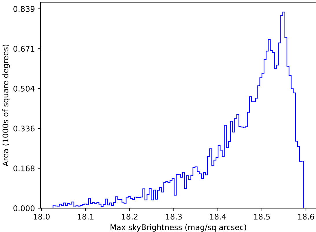
too_10_1v3.4_10yrs Yr 1 y band: Max skyBrightness
