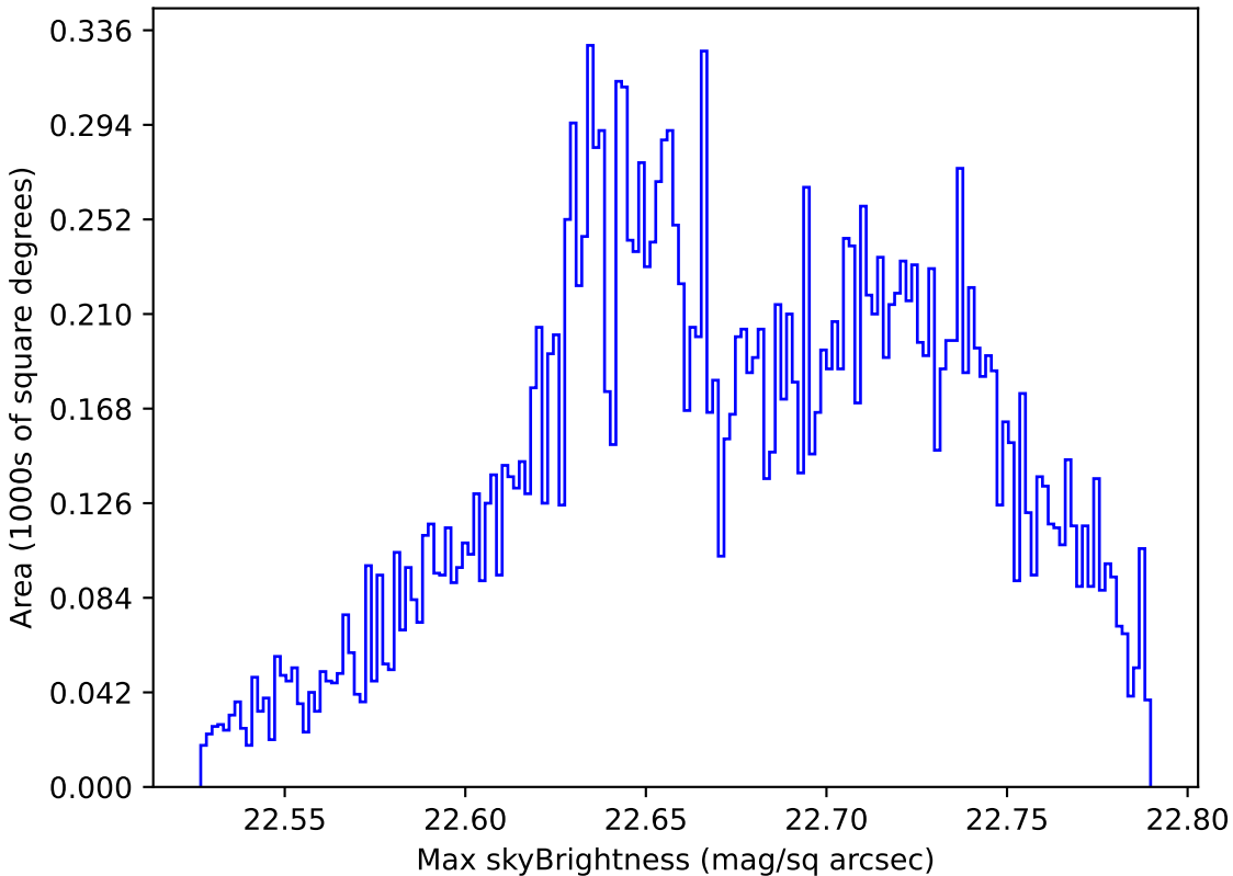
too_10_1v3.4_10yrs Yr 1 u band: Max skyBrightness
