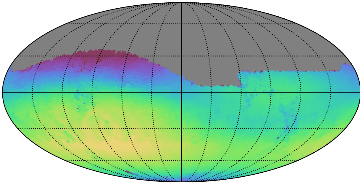
too_10_1v3.4_10yrs Yr 1 r band: Max skyBrightness
