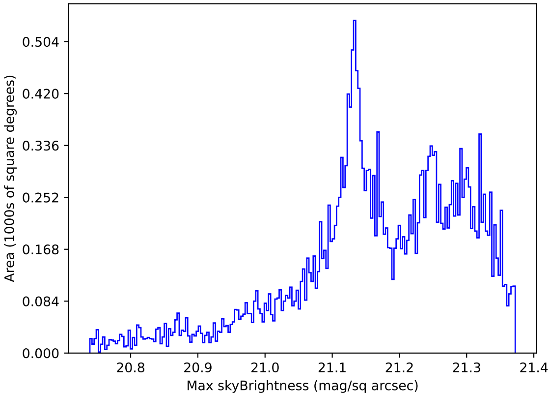
too_10_1v3.4_10yrs Yr 1 r band: Max skyBrightness
