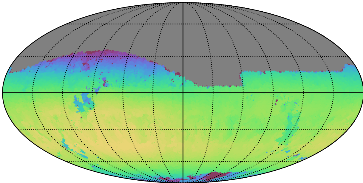
too_10_1v3.4_10yrs Yr 1 i band: Max skyBrightness
