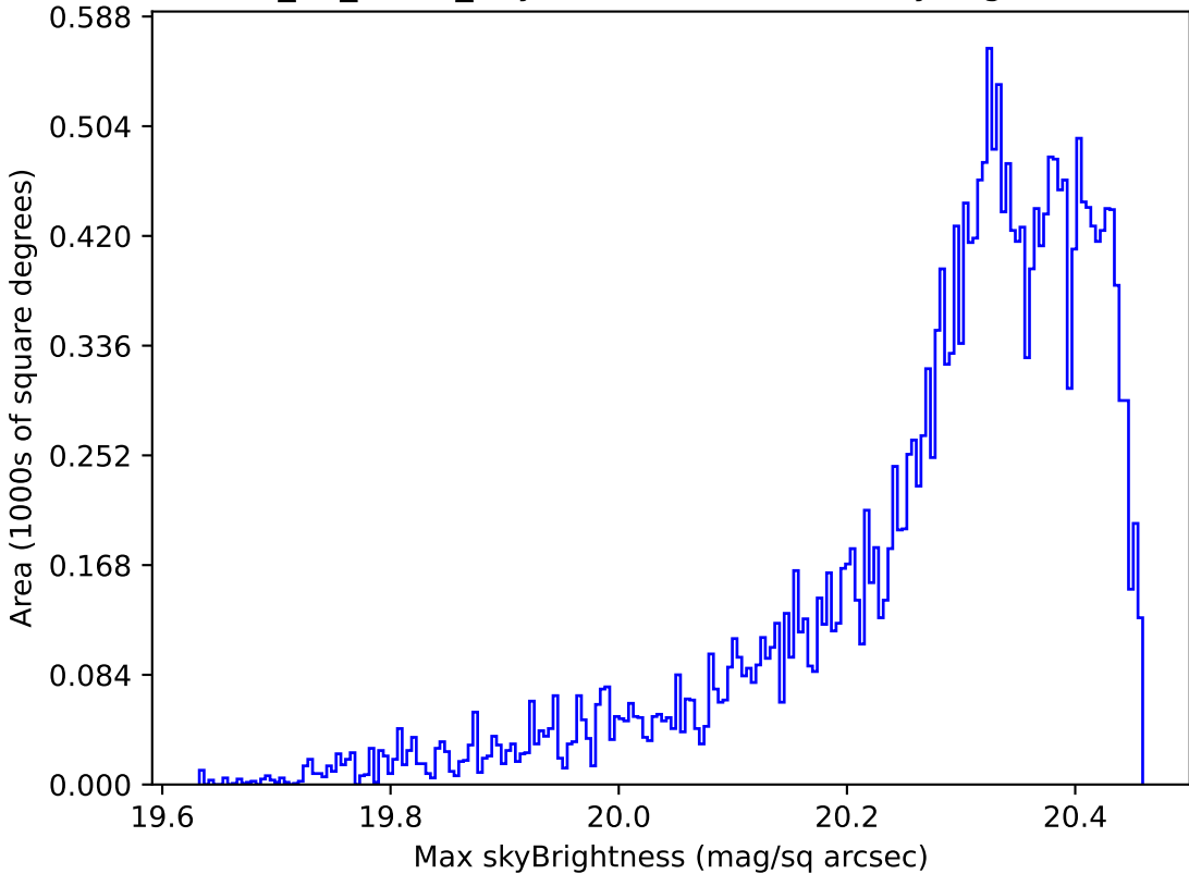
too_10_1v3.4_10yrs Yr 1 i band: Max skyBrightness
