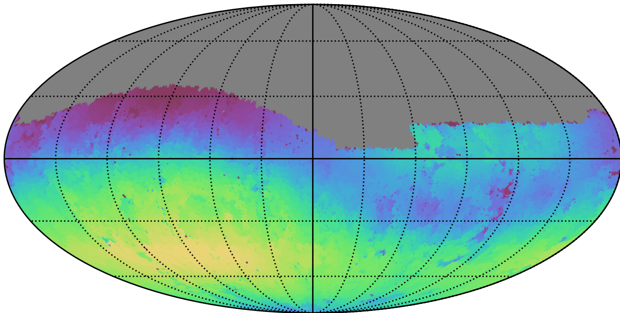
too_10_1v3.4_10yrs Yr 1 g band: Max skyBrightness
