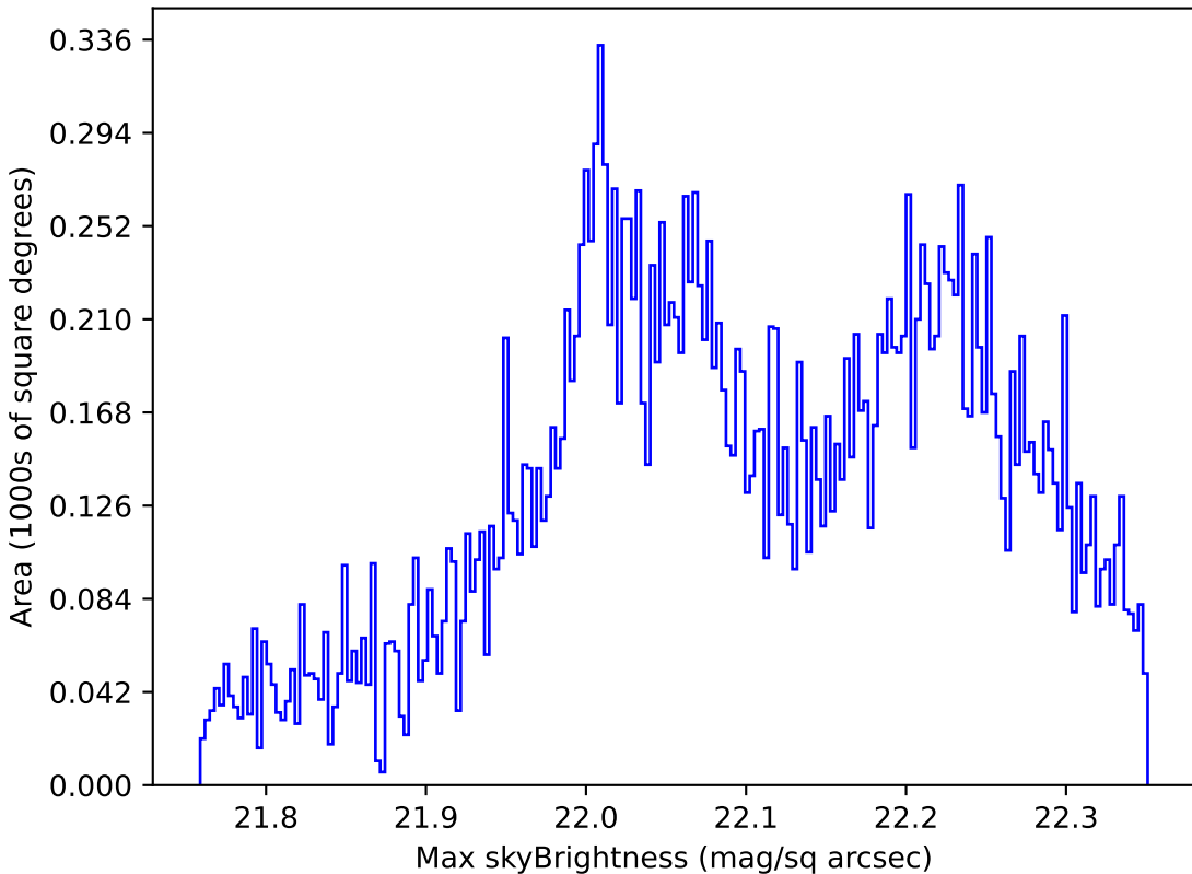
too_10_1v3.4_10yrs Yr 1 g band: Max skyBrightness
