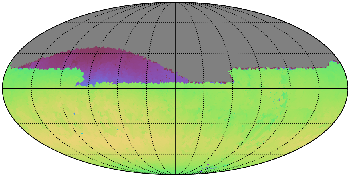
too_10_1v3.4_10yrs Yr 1 all bands: Max skyBrightness
