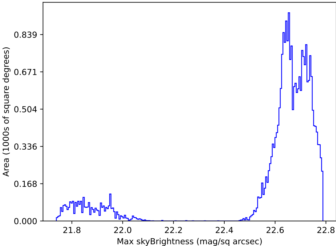
too_10_1v3.4_10yrs Yr 1 all bands: Max skyBrightness
