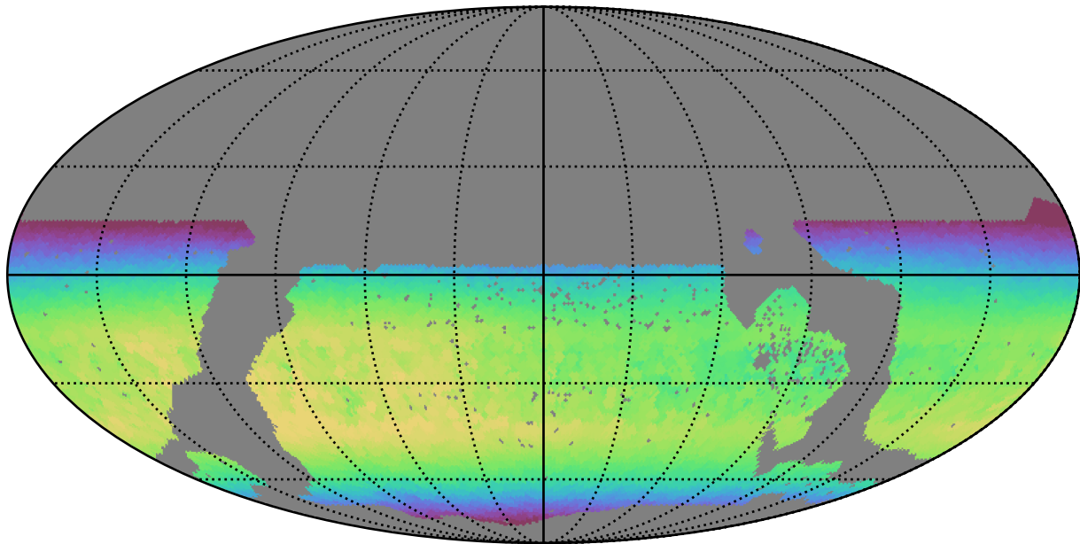
too_10_1v3.4_10yrs WFD z band: Max skyBrightness
