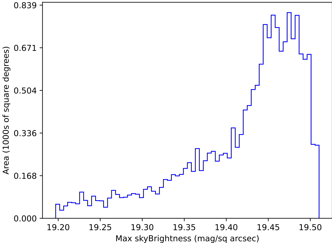
too_10_1v3.4_10yrs WFD z band: Max skyBrightness
