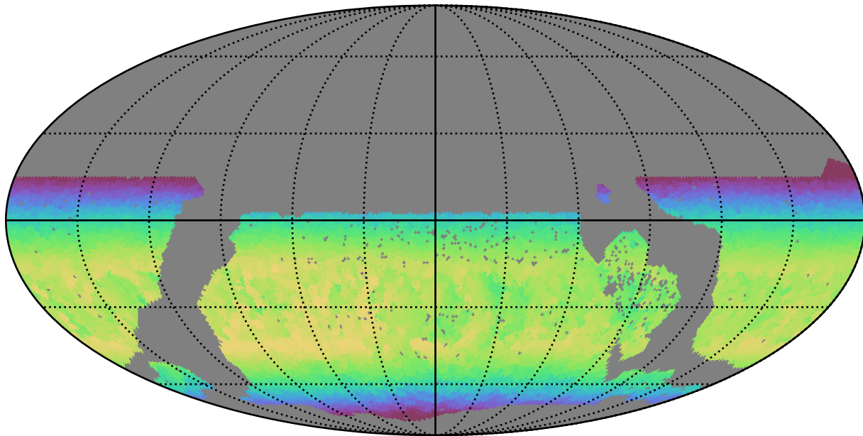
too_10_1v3.4_10yrs WFD y band: Max skyBrightness
