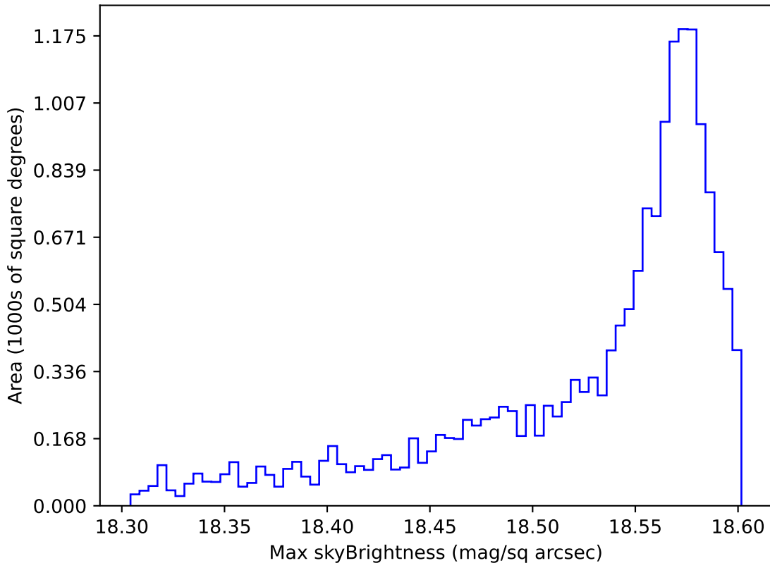
too_10_1v3.4_10yrs WFD y band: Max skyBrightness
