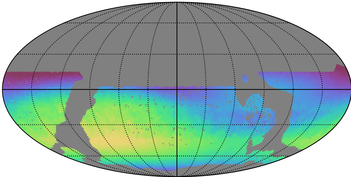
too_10_1v3.4_10yrs WFD u band: Max skyBrightness
