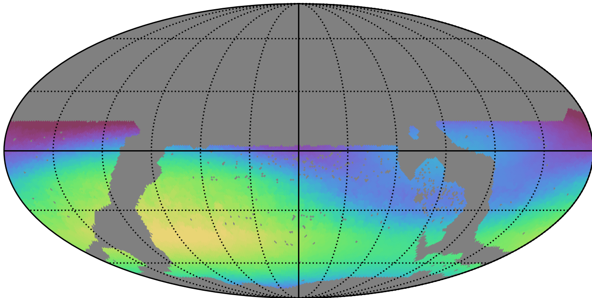
too_10_1v3.4_10yrs WFD r band: Max skyBrightness
