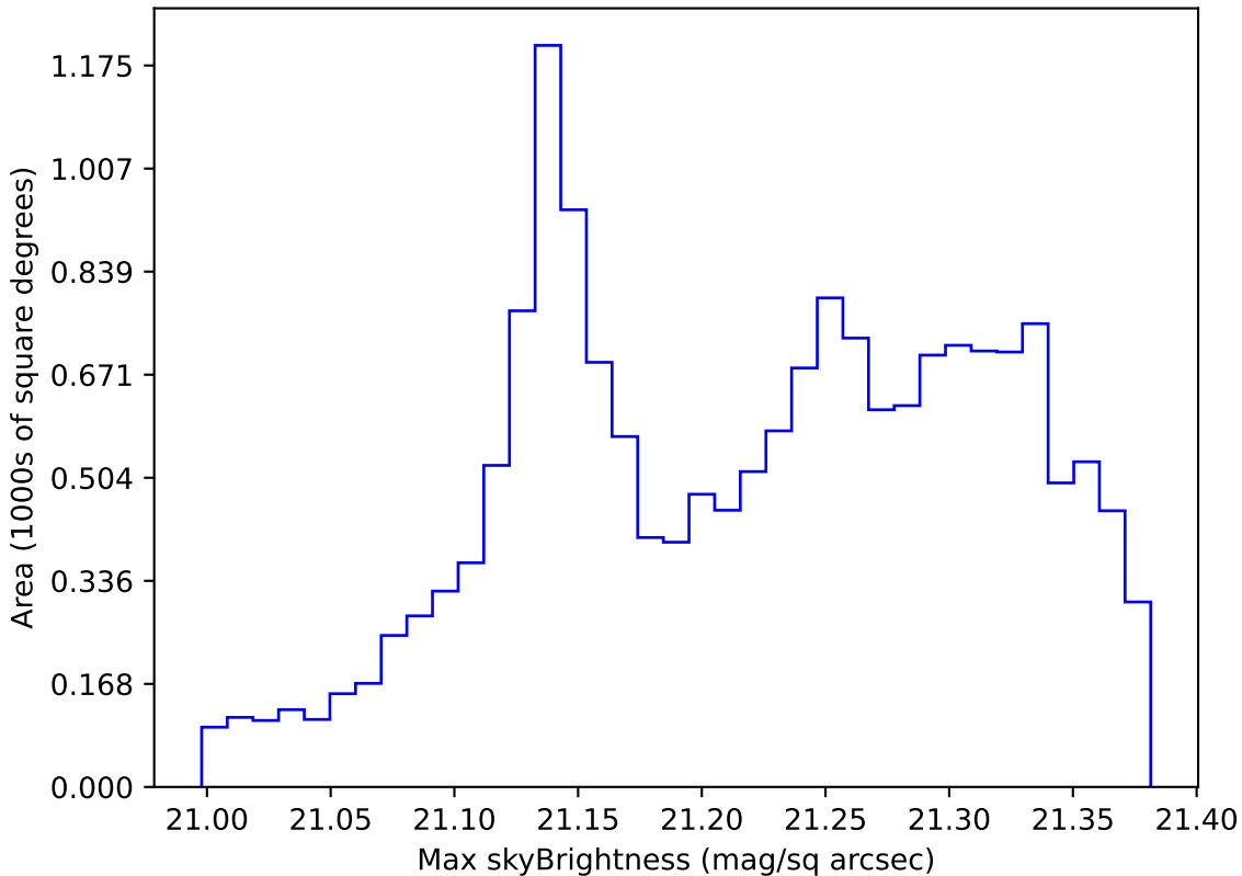
too_10_1v3.4_10yrs WFD r band: Max skyBrightness
