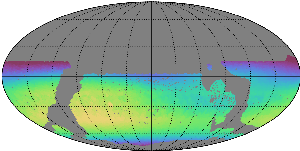
too_10_1v3.4_10yrs WFD i band: Max skyBrightness
