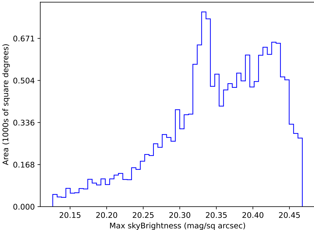
too_10_1v3.4_10yrs WFD i band: Max skyBrightness
