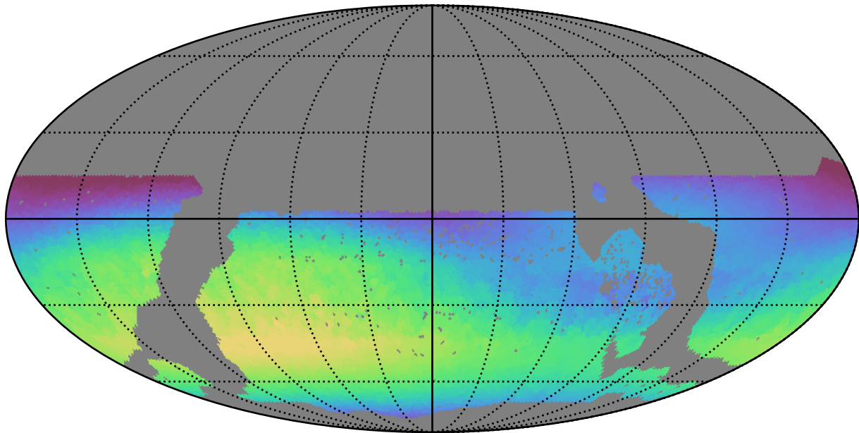
too_10_1v3.4_10yrs WFD all bands: Max skyBrightness
