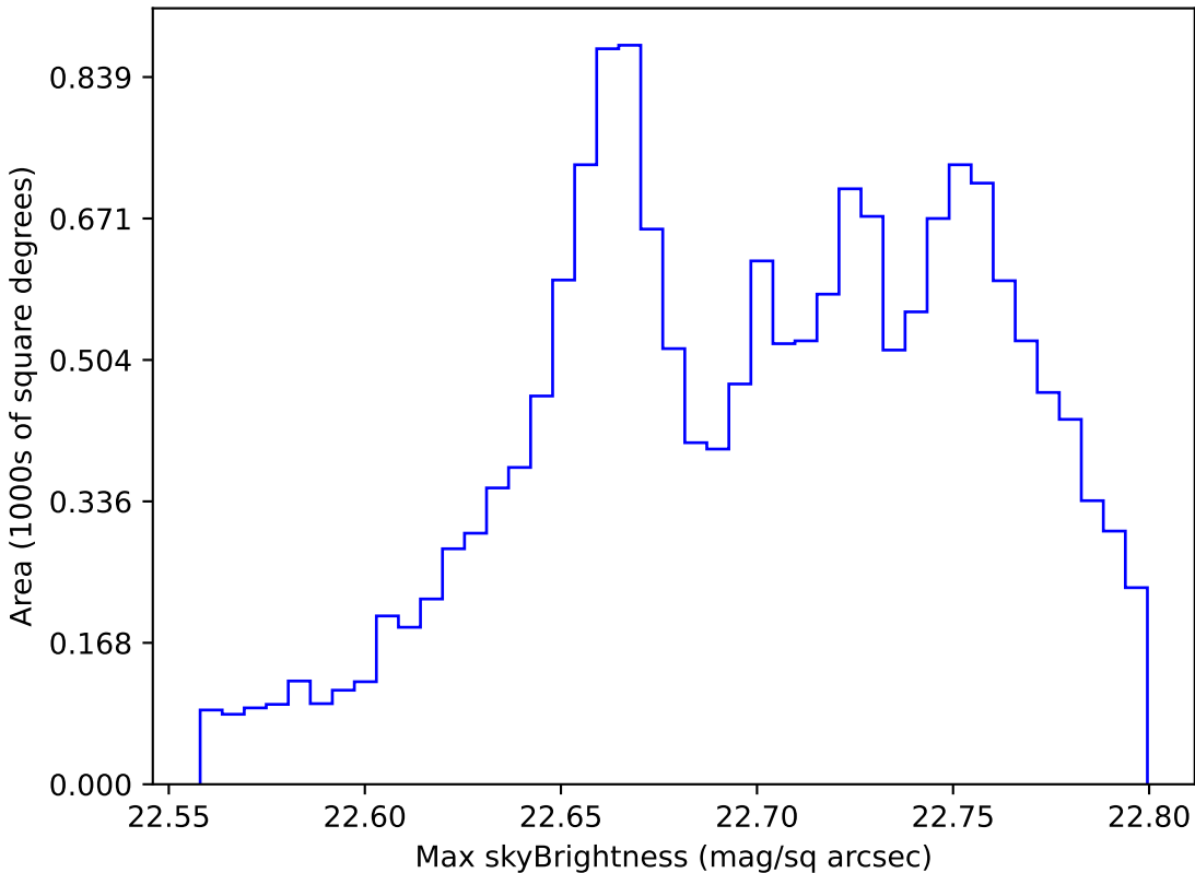
too_10_1v3.4_10yrs WFD all bands: Max skyBrightness
