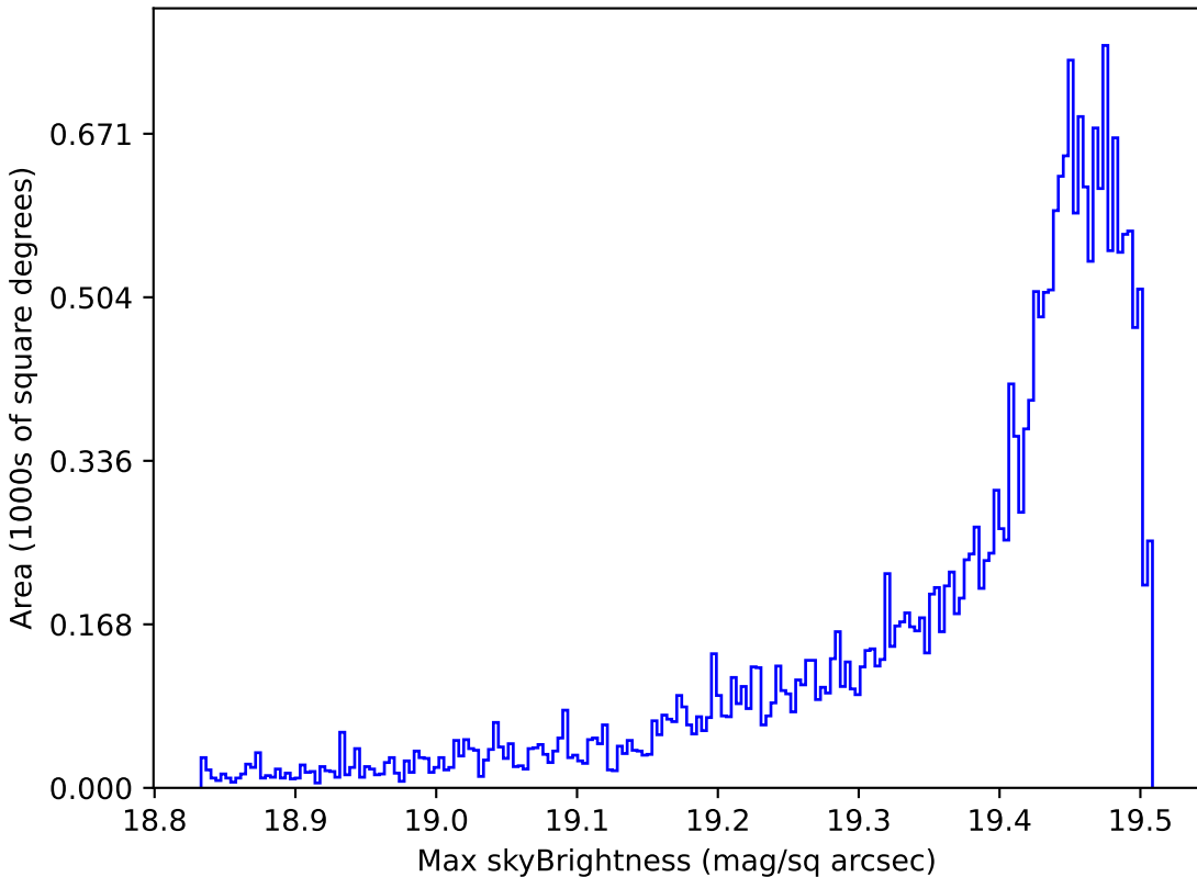
too_10_1v3.4_10yrs All sky z band: Max skyBrightness
