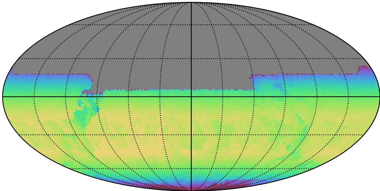
too_10_1v3.4_10yrs All sky y band: Max skyBrightness
