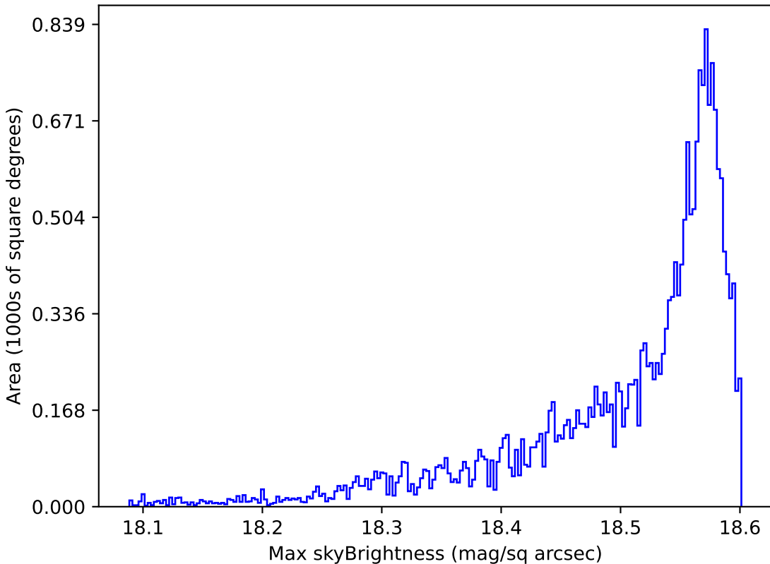
too_10_1v3.4_10yrs All sky y band: Max skyBrightness
