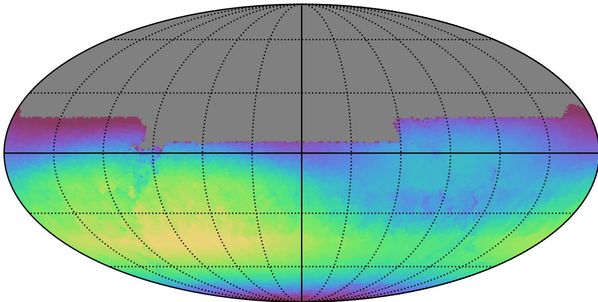
too_10_1v3.4_10yrs All sky u band: Max skyBrightness
