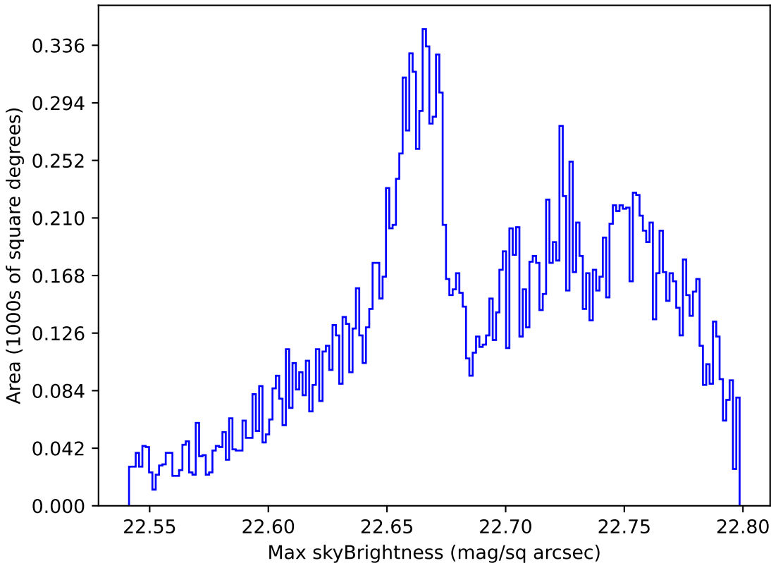
too_10_1v3.4_10yrs All sky u band: Max skyBrightness
