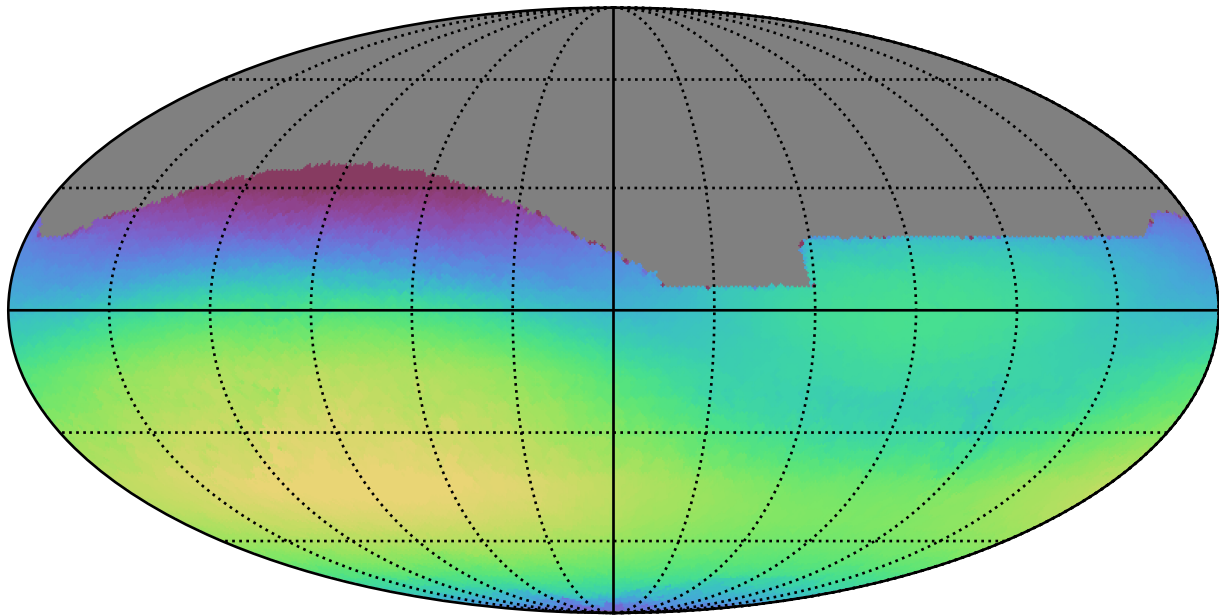
too_10_1v3.4_10yrs All sky r band: Max skyBrightness
