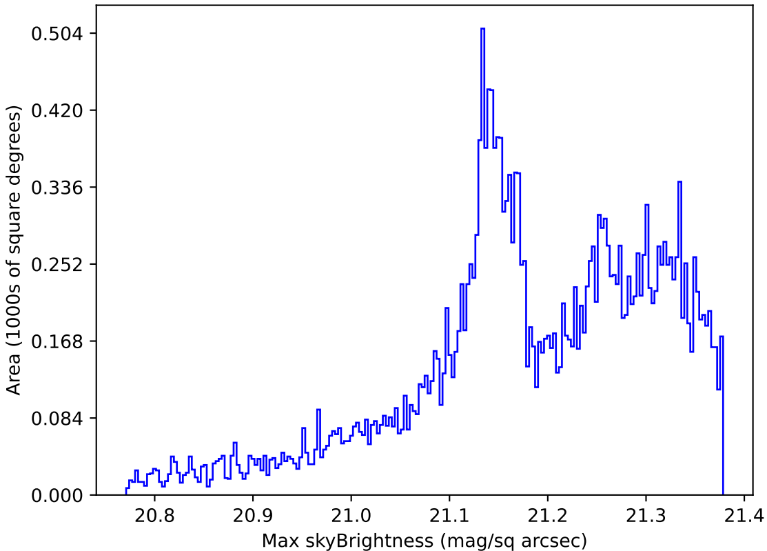
too_10_1v3.4_10yrs All sky r band: Max skyBrightness
