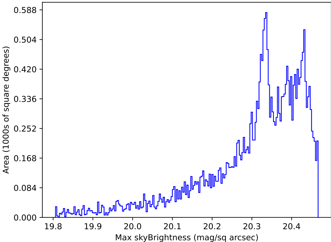
too_10_1v3.4_10yrs All sky i band: Max skyBrightness
