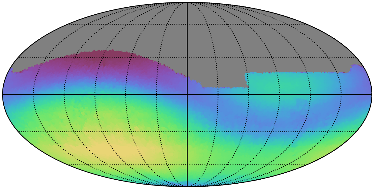
too_10_1v3.4_10yrs All sky g band: Max skyBrightness
