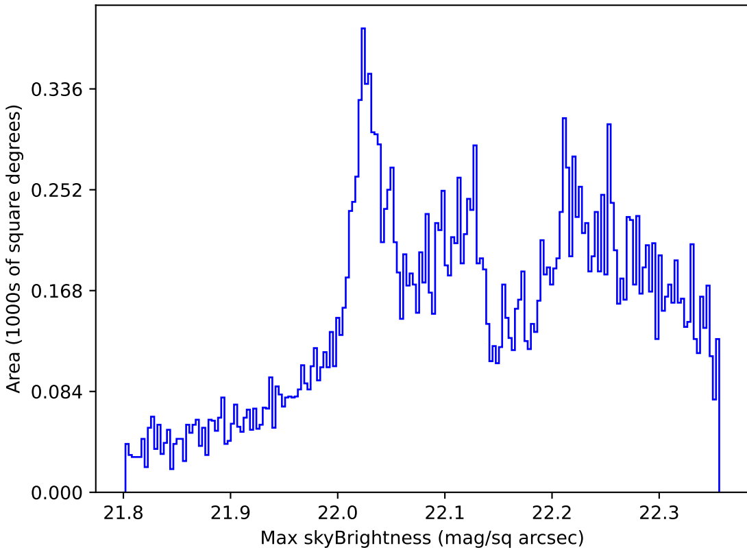
too_10_1v3.4_10yrs All sky g band: Max skyBrightness
