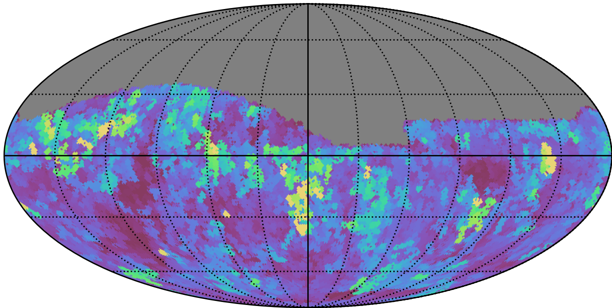
too_10_1v3.4_10yrs Yr 1 z band: Max seeingGeom
