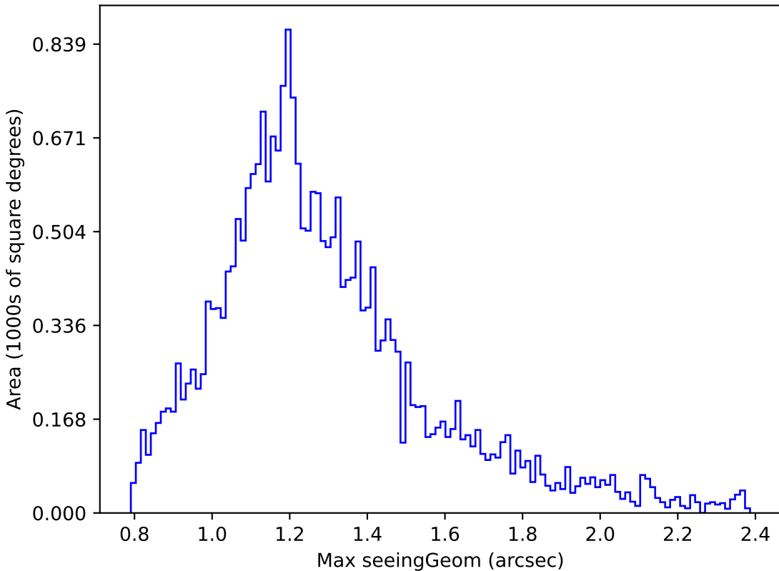
too_10_1v3.4_10yrs Yr 1 z band: Max seeingGeom
