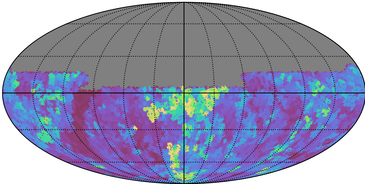
too_10_1v3.4_10yrs Yr 1 y band: Max seeingGeom
