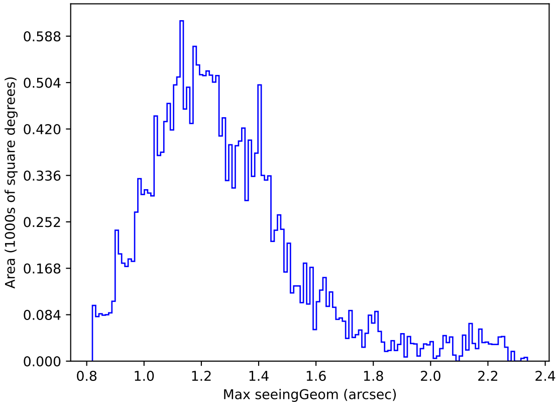
too_10_1v3.4_10yrs Yr 1 y band: Max seeingGeom
