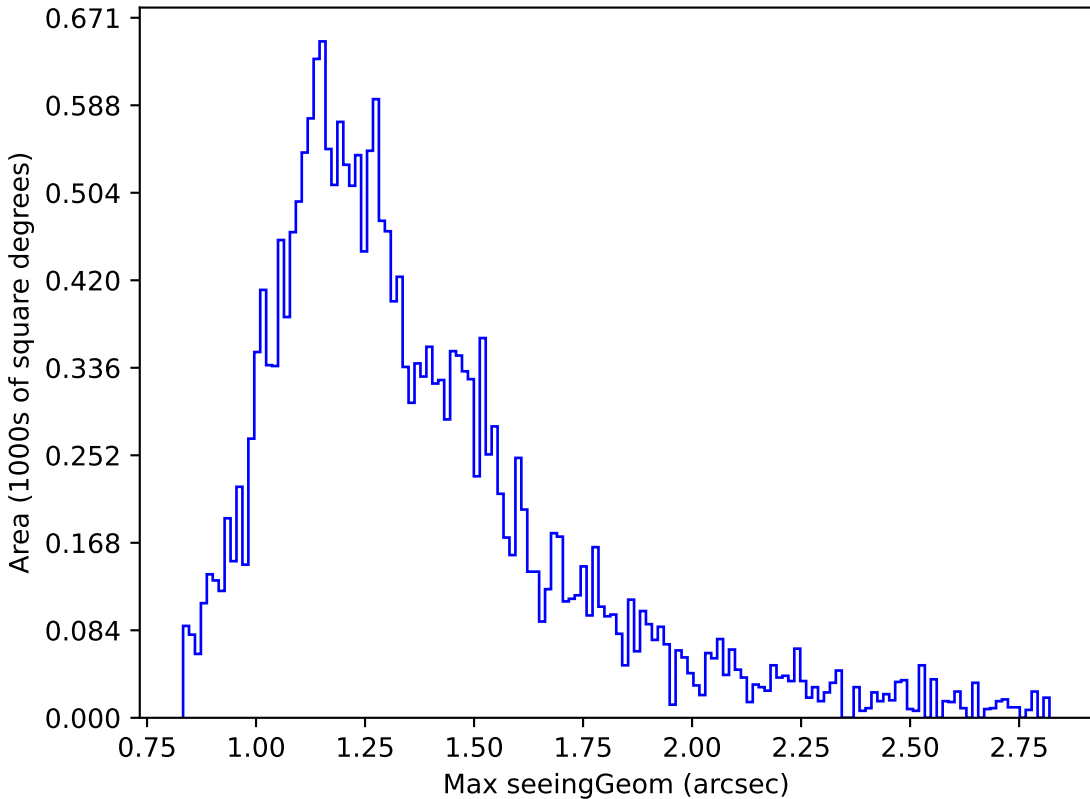
too_10_1v3.4_10yrs Yr 1 u band: Max seeingGeom
