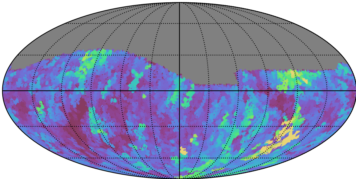
too_10_1v3.4_10yrs Yr 1 r band: Max seeingGeom
