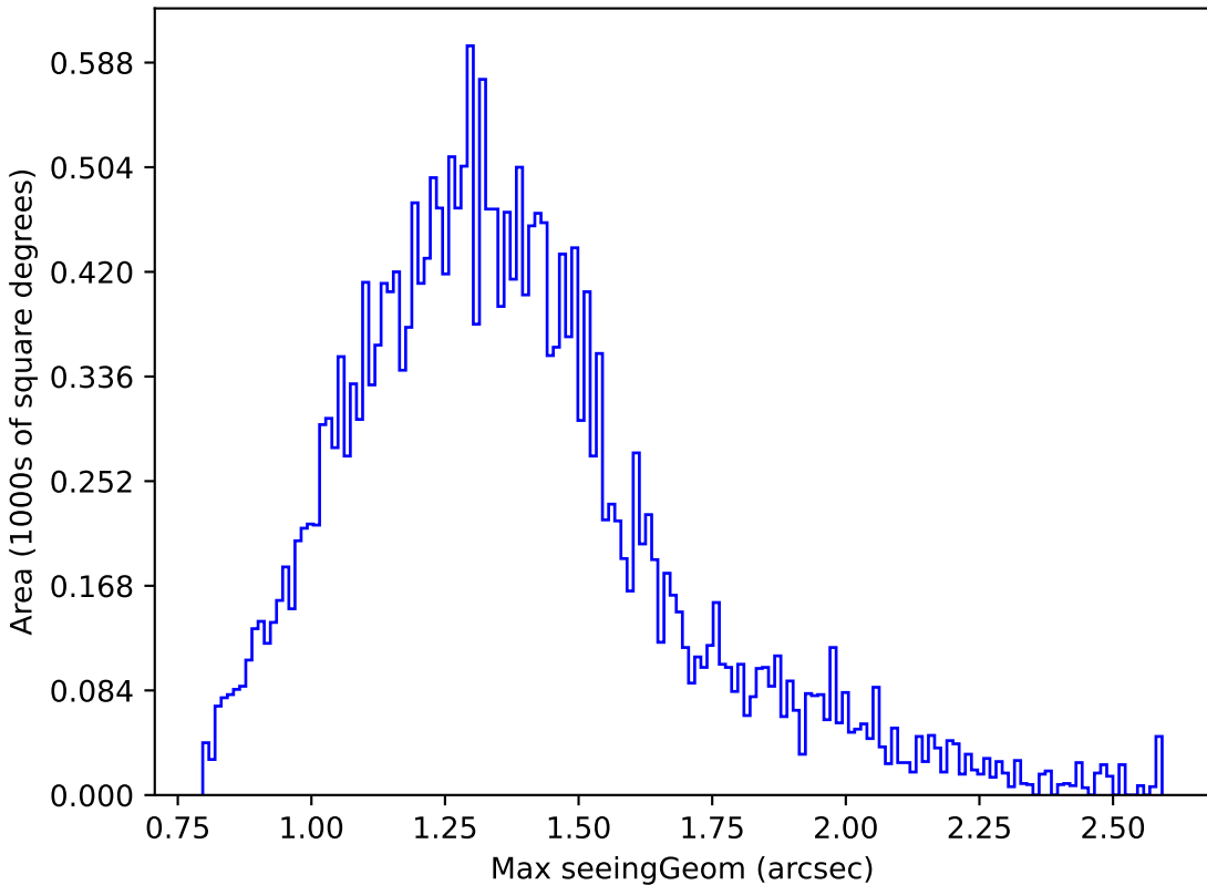
too_10_1v3.4_10yrs Yr 1 r band: Max seeingGeom
