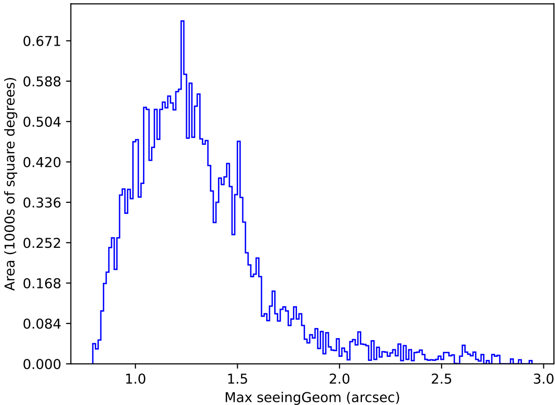
too_10_1v3.4_10yrs Yr 1 i band: Max seeingGeom
