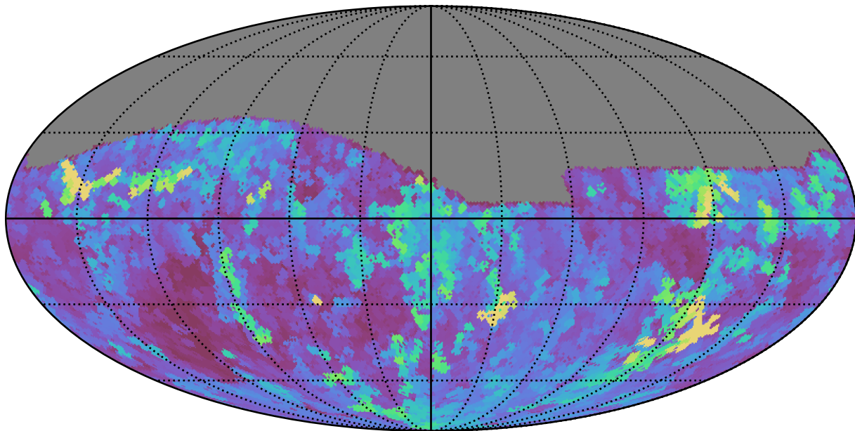
too_10_1v3.4_10yrs Yr 1 all bands: Max seeingGeom
